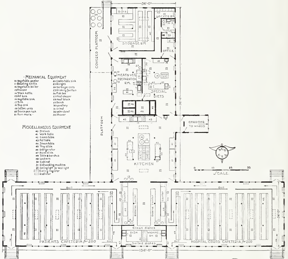
• GENERAL KITCHEN & MESS • [34] •
